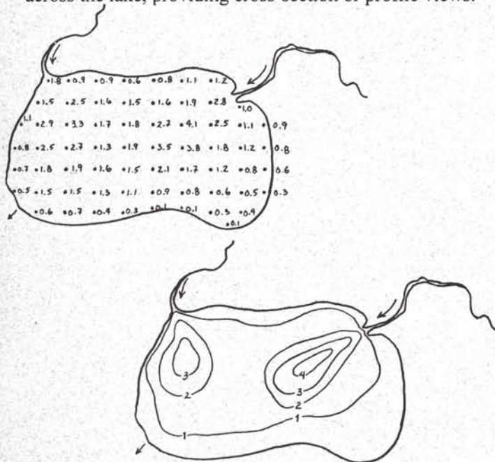
Lake sediment thickness measurements and resulting contour map (arrows indicate inflowing and outflowing streams).
