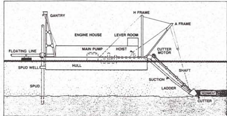
Configuration of a typical cutterhead dredge.
